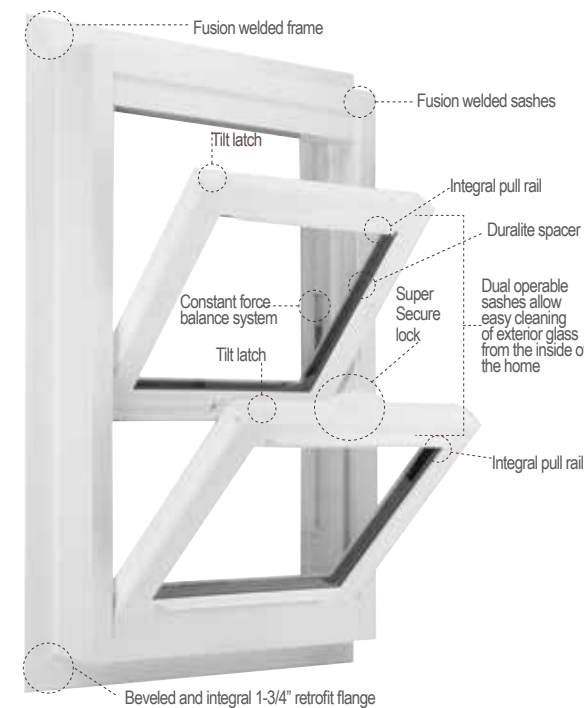
DOUBLE HUNG
