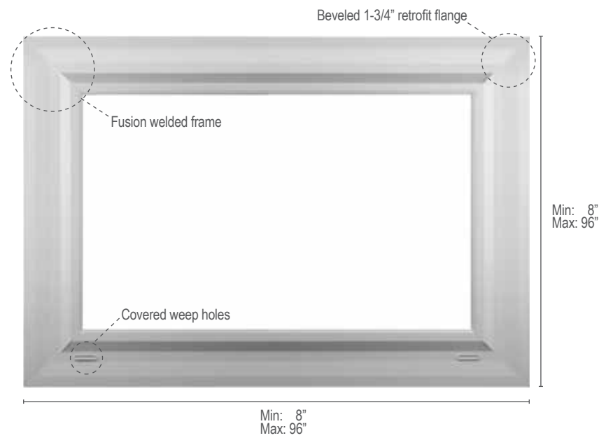
PICTURE WINDOW
